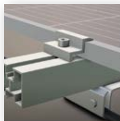
Use the end clamp and use it to attach the panel to the structure, screw the clamp with an allen screw and square nut
